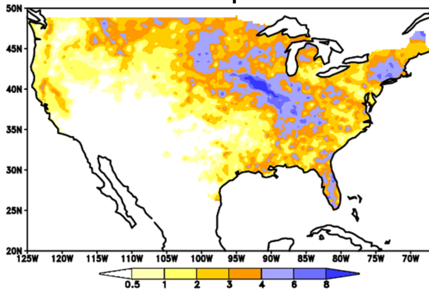
GTS Precipitation
